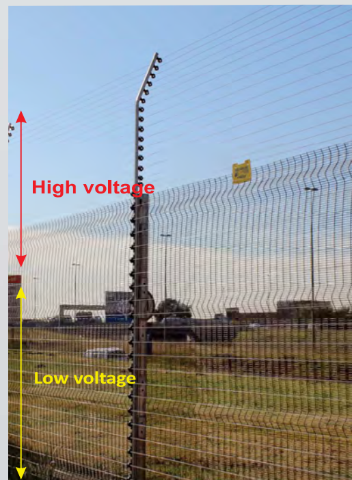
ZLM4 Used to Make Fence IEC 60335 / AS/NZS 3016 Compliant
